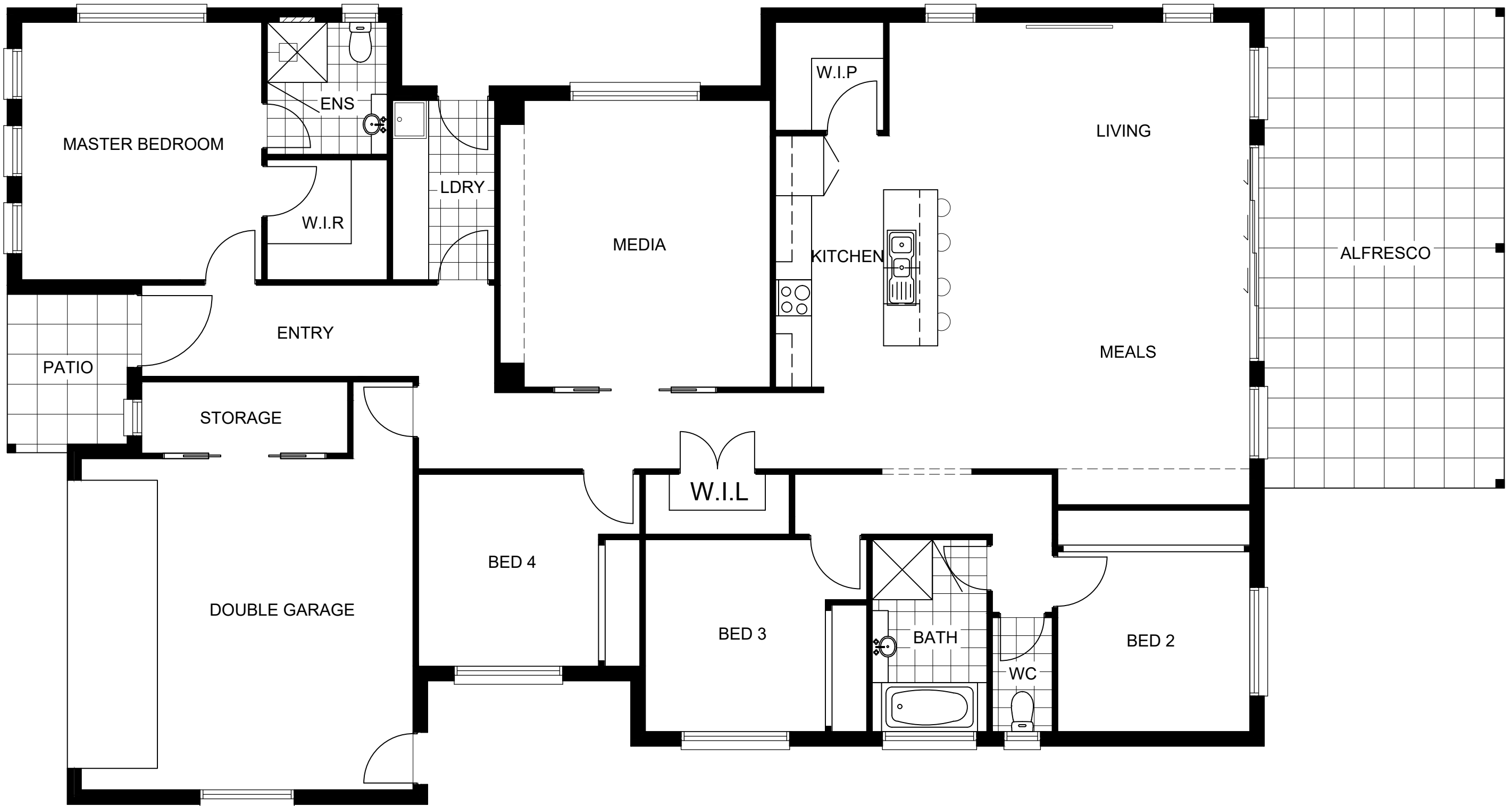
FLOOR PLAN
